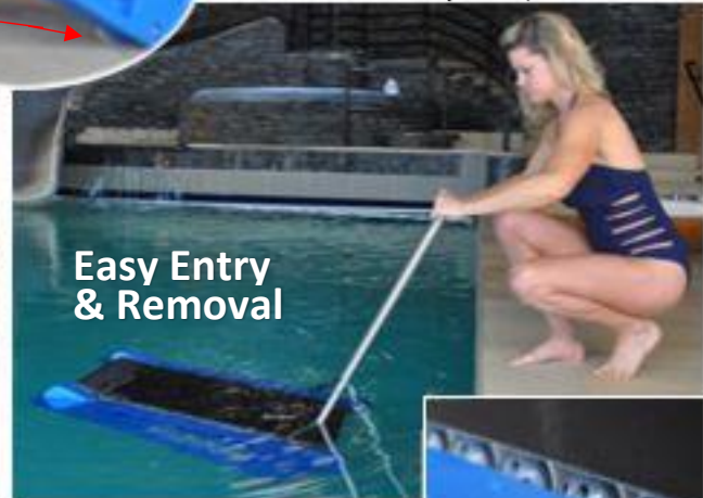
Constructed of Polyethylene, ABS, PVC, and Stainless Steel so that it Can Stay in the Pool Year-round with No Damage
